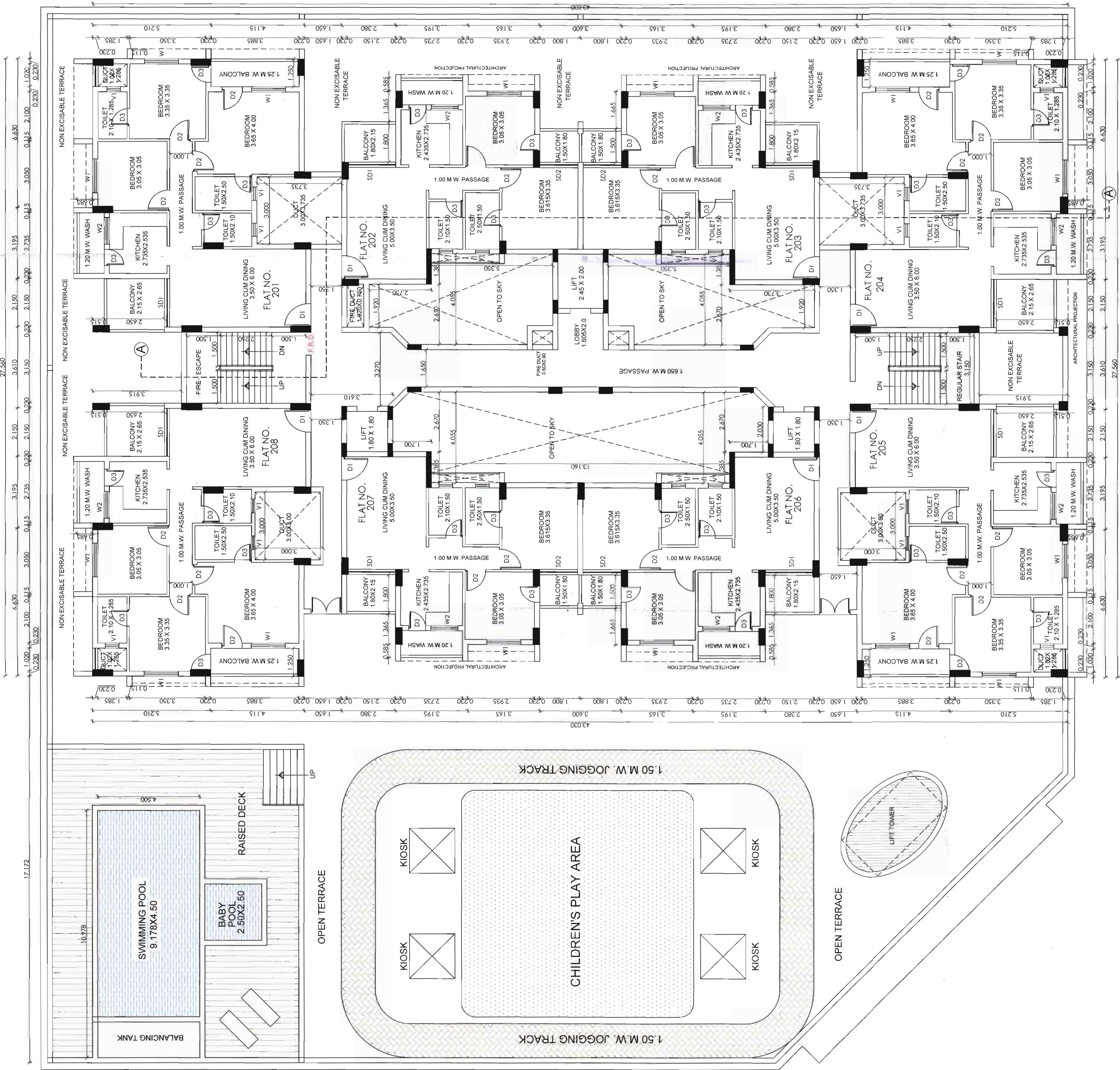
2ND FLOOR PLAN SCALE:- 1:100
