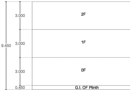
SECTION VIEW - BLOCK A
