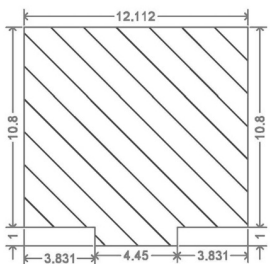
BUILT-UP AREA CALCULATION GROUND FLOOR BLOCK A
