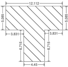
BUILT-UP AREA CALCULATION SECOND FLOOR BLOCK A
