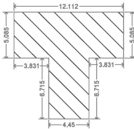
BUILT-UP AREA CALCULATION SECOND FLOOR BLOCK A
