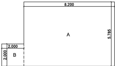
GROUND FLOOR PLAN (ROW HOUSE NO. 101) SCALE 1:100
