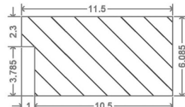
BUILT-UP AREA CALCULATION GROUND FLOOR BLOCK F
