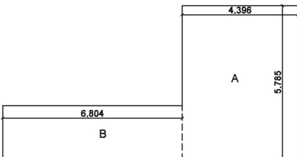
SECOND FLOOR PLAN (ROW HOUSE NO. 101) SCALE 1:100
