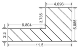
BUILT-UP AREA CALCULATION SECOND FLOOR BLOCK F
