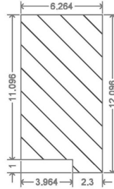
BUILT-UP AREA CALCULATION GROUND FLOOR BLOCK F
