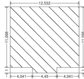
BUILT-UP AREA CALCULATION GROUND FLOOR BLOCK F
