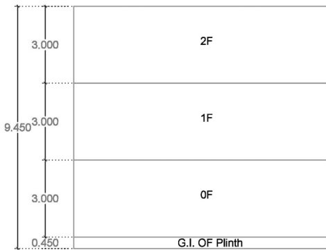
SECTION VIEW - BLOCK F
