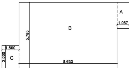
FIRST FLOOR PLAN (ROW HOUSE NO. 101) SCALE 1:100
