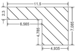
BUILT-UP AREA CALCULATION SECOND FLOOR BLOCK F
