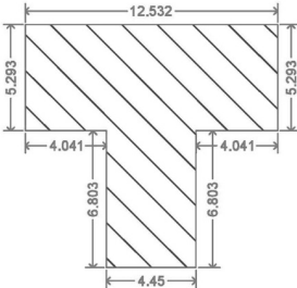
BUILT-UP AREA CALCULATION SECOND FLOOR BLOCK F
