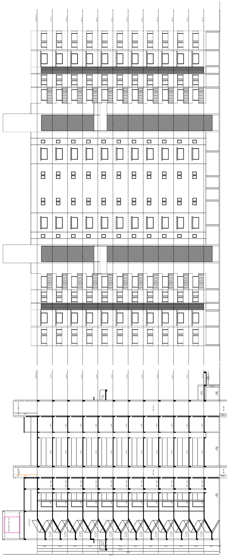
FRONT ELEVATION
