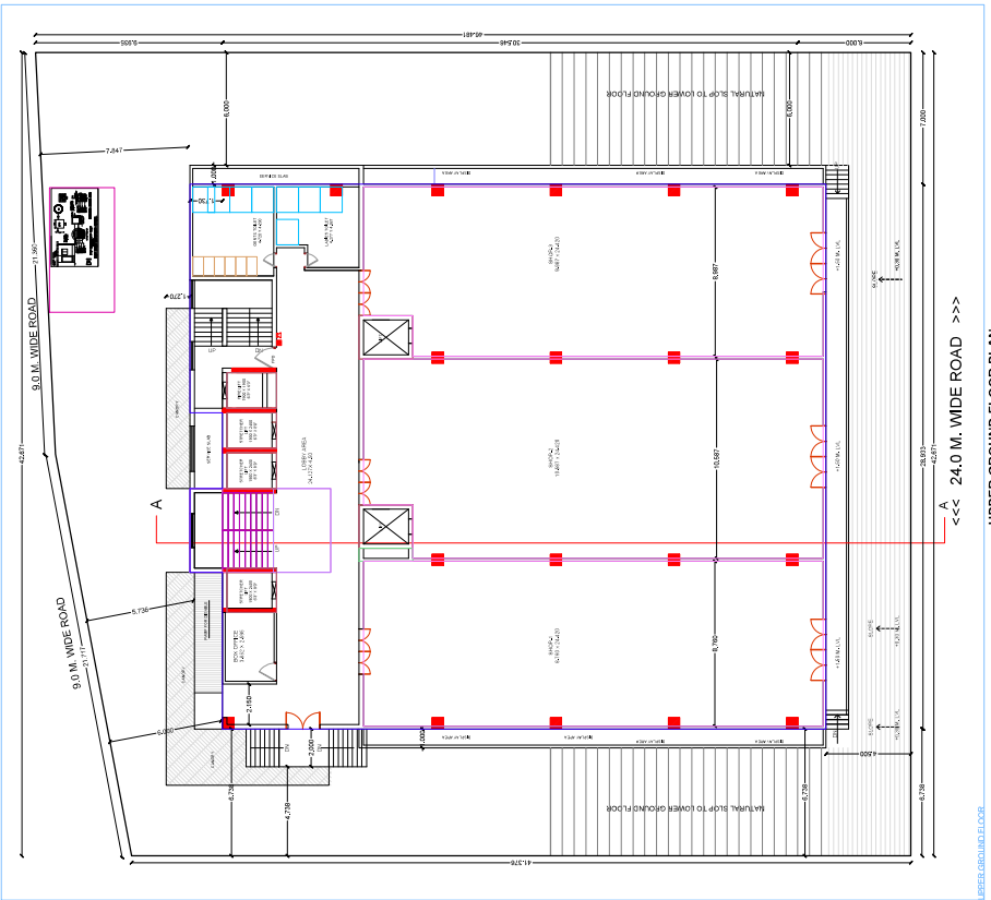
UPPER GROUND FLOOR PLAN SCALE 1:100
