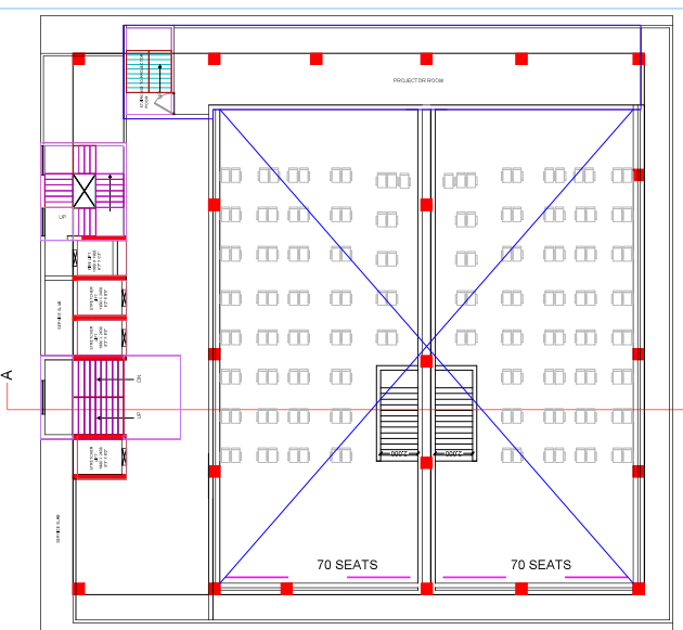
PROJECTOR ROOM PLAN SCALE 1:100
