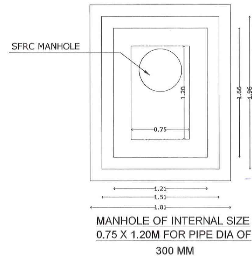
C / S DETAILS OF SEWER LINE CHAMBERS FOR NAGPUR METROPOLITAN AREA
