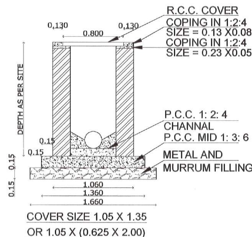
PROPOSED DEVELOPMENT DRAWING FOR SEWER LINES
