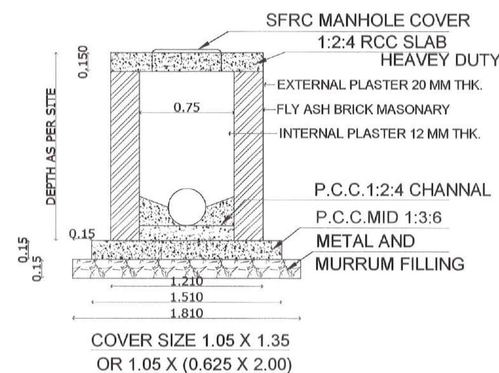
PROPOSED DEVELOPMENT DRAWING FOR SEWER LINES
