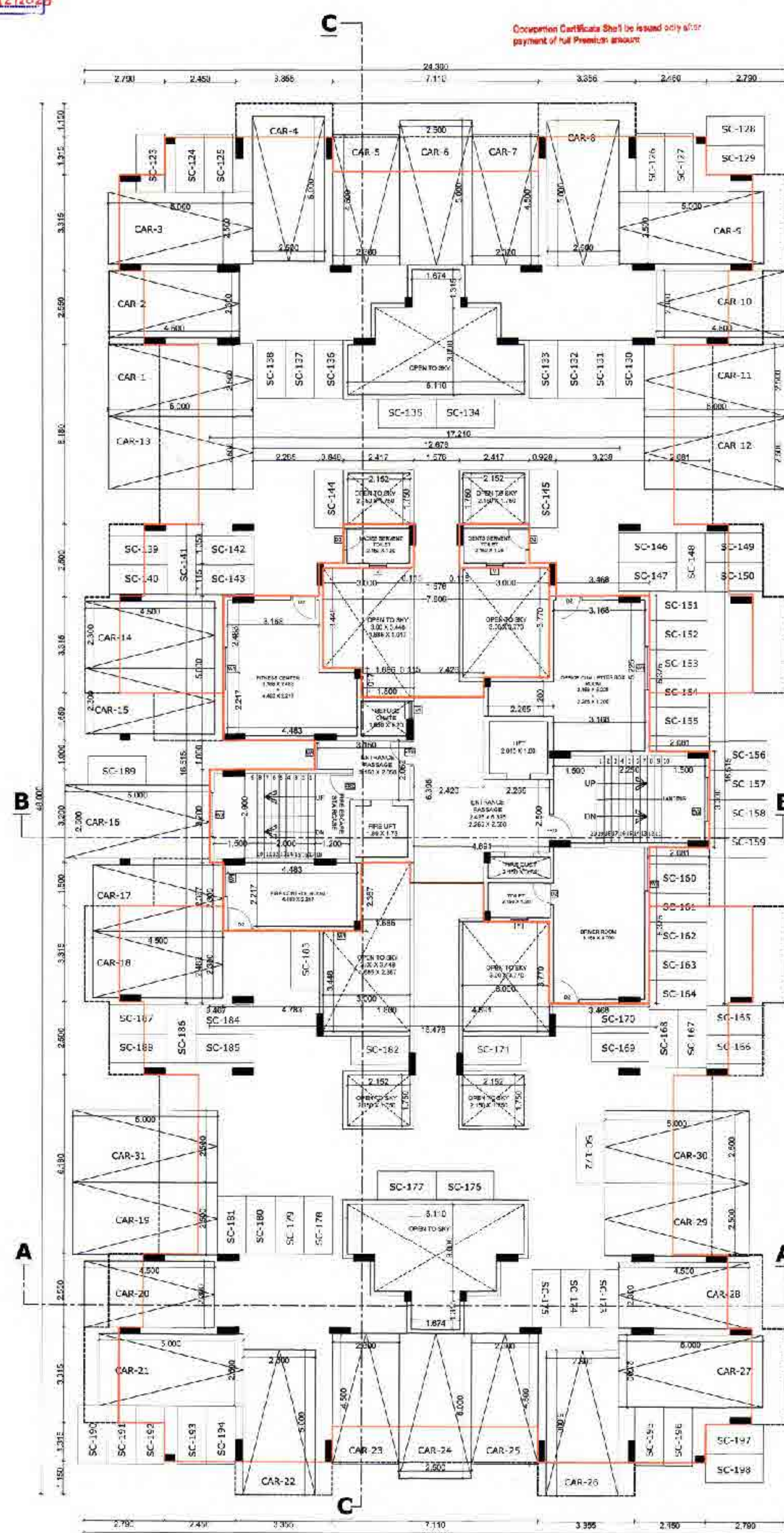
TOWER - A EXISTING GROUND FLOOR PLAN
