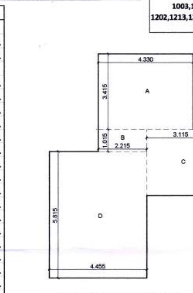
CARPET AREA KEY PLAN FOR FLAT NO. 204 (WING-E) SCALE - 1:100
