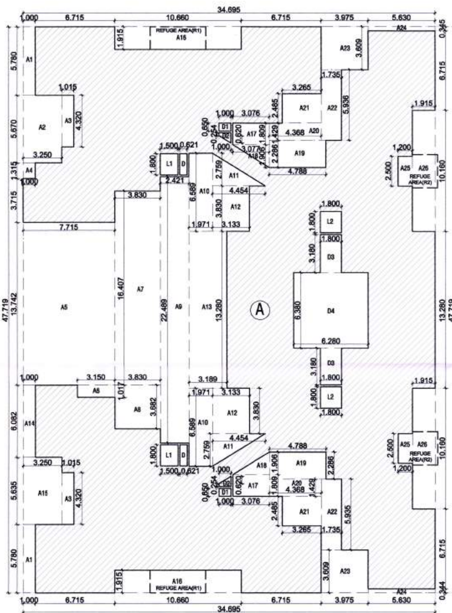
B/U/P AREA KEY PLAN EIGHTH FLOOR PLAN (WING-E) SCALE - 1:200
