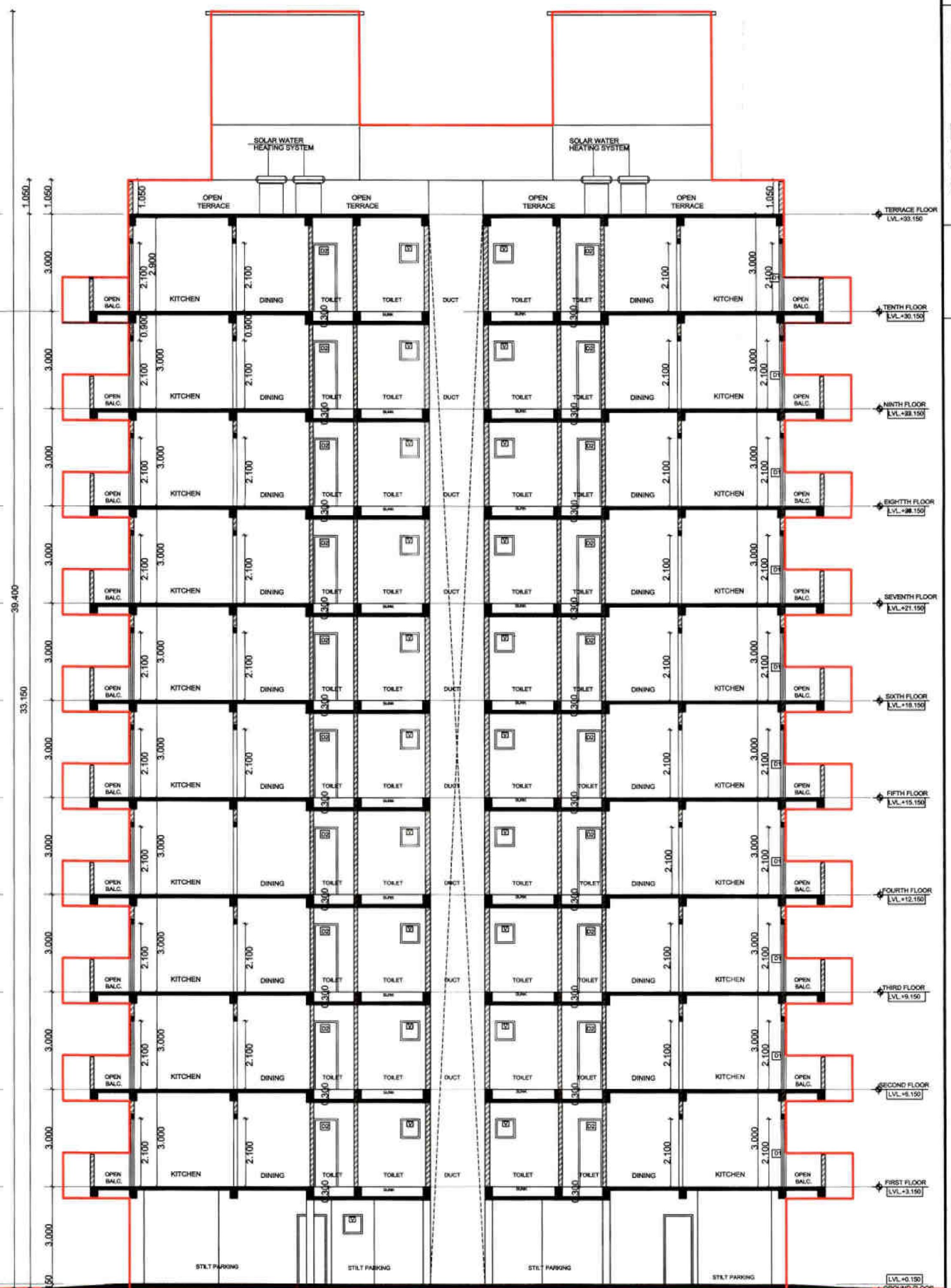
SECTION A-A BUILDING - 2 (TOWER - B)
