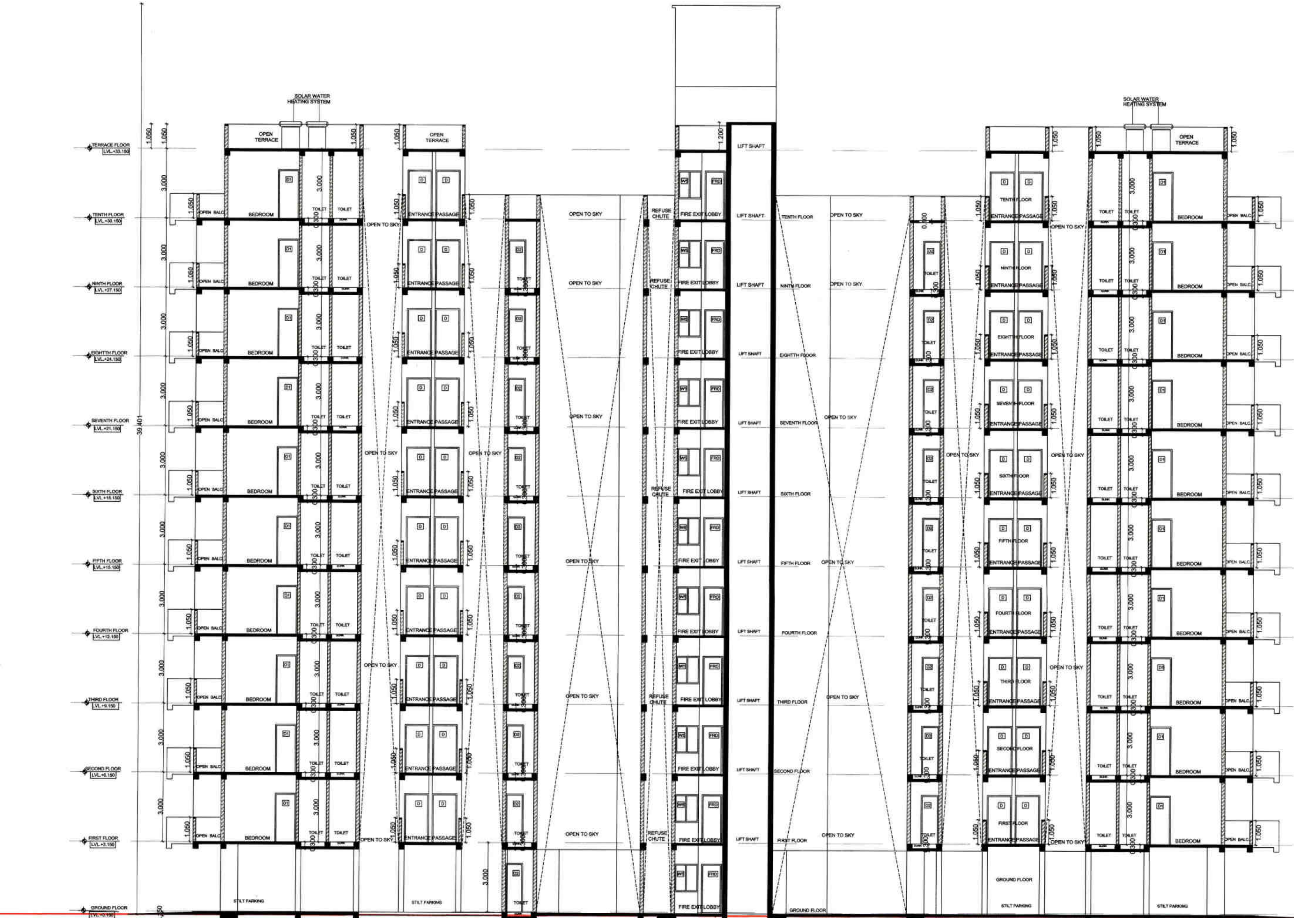
SECTION C-C BUILDING - 2 (TOWER - B)
