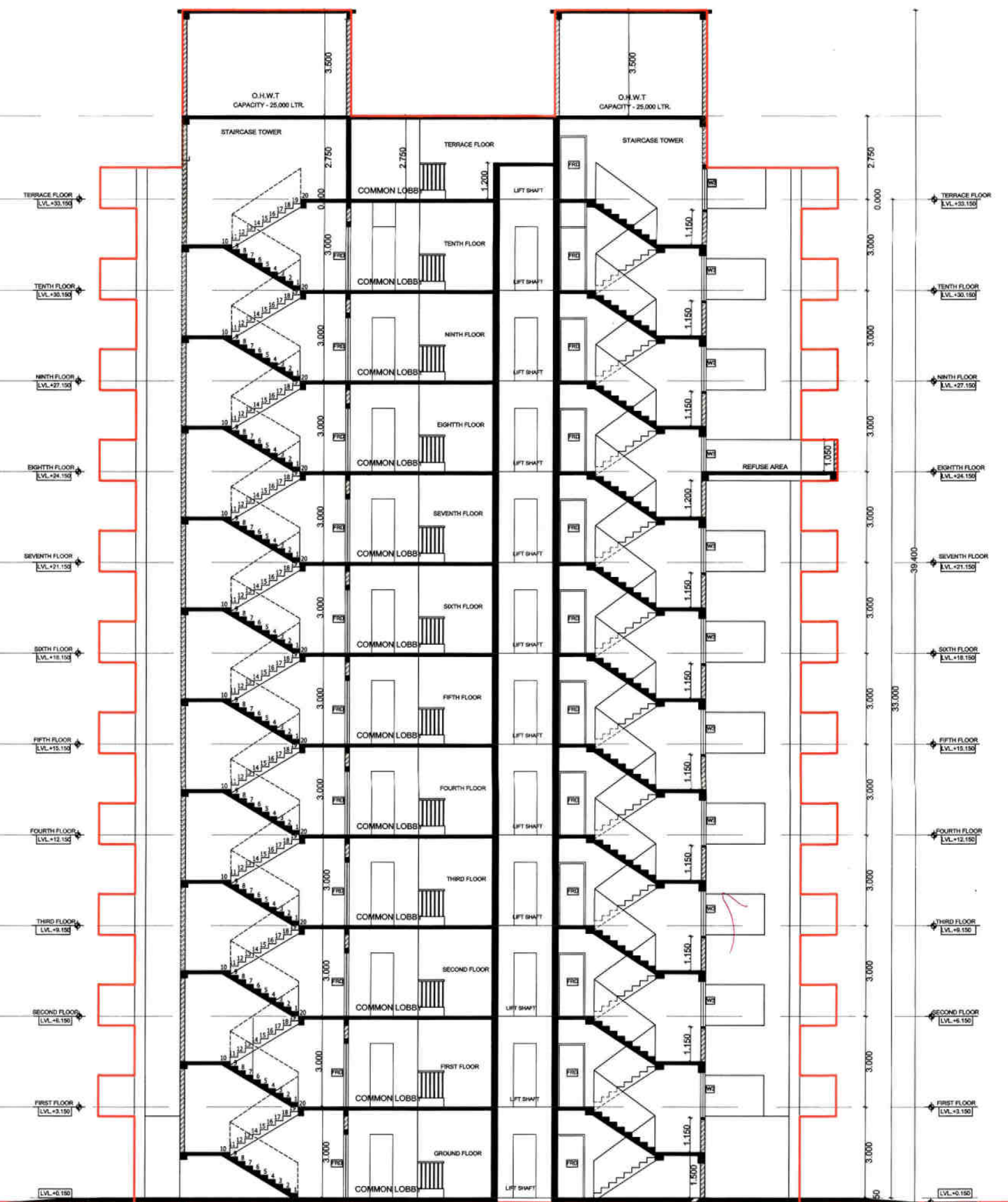
SECTION B-B BUILDING - 2 (TOWER - B)
