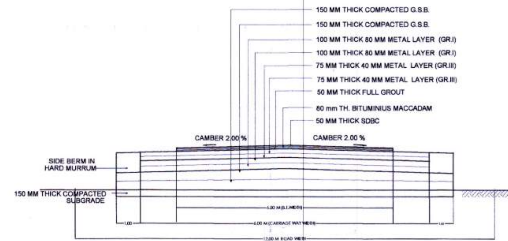
CROSS SECTION OF 12.00 M WIDE ROAD
