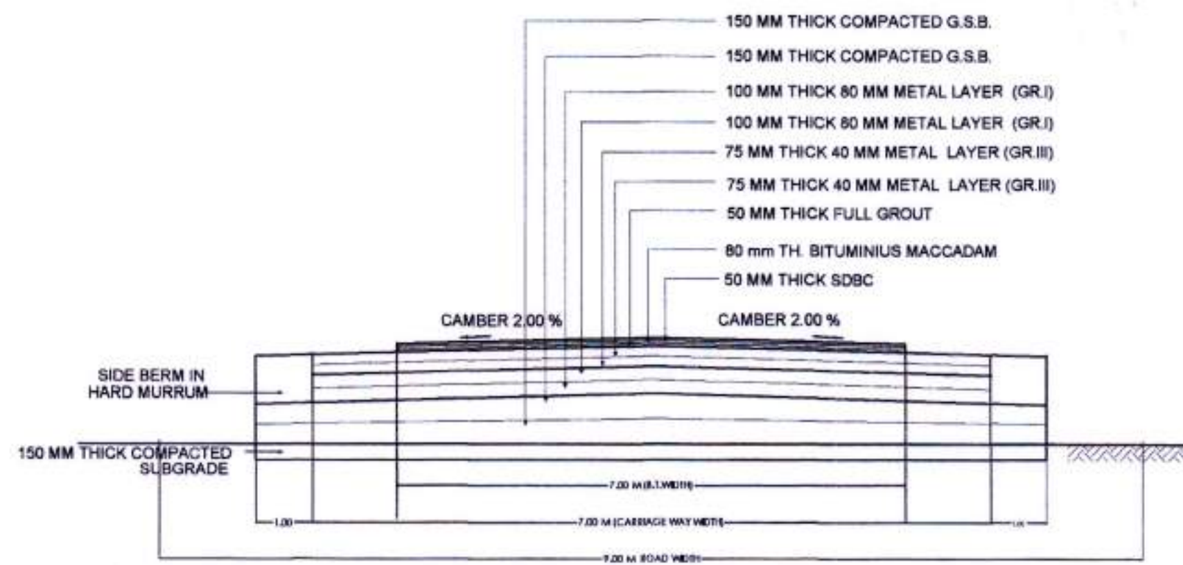
CROSS SECTION OF 9.00 M WIDE ROAD
