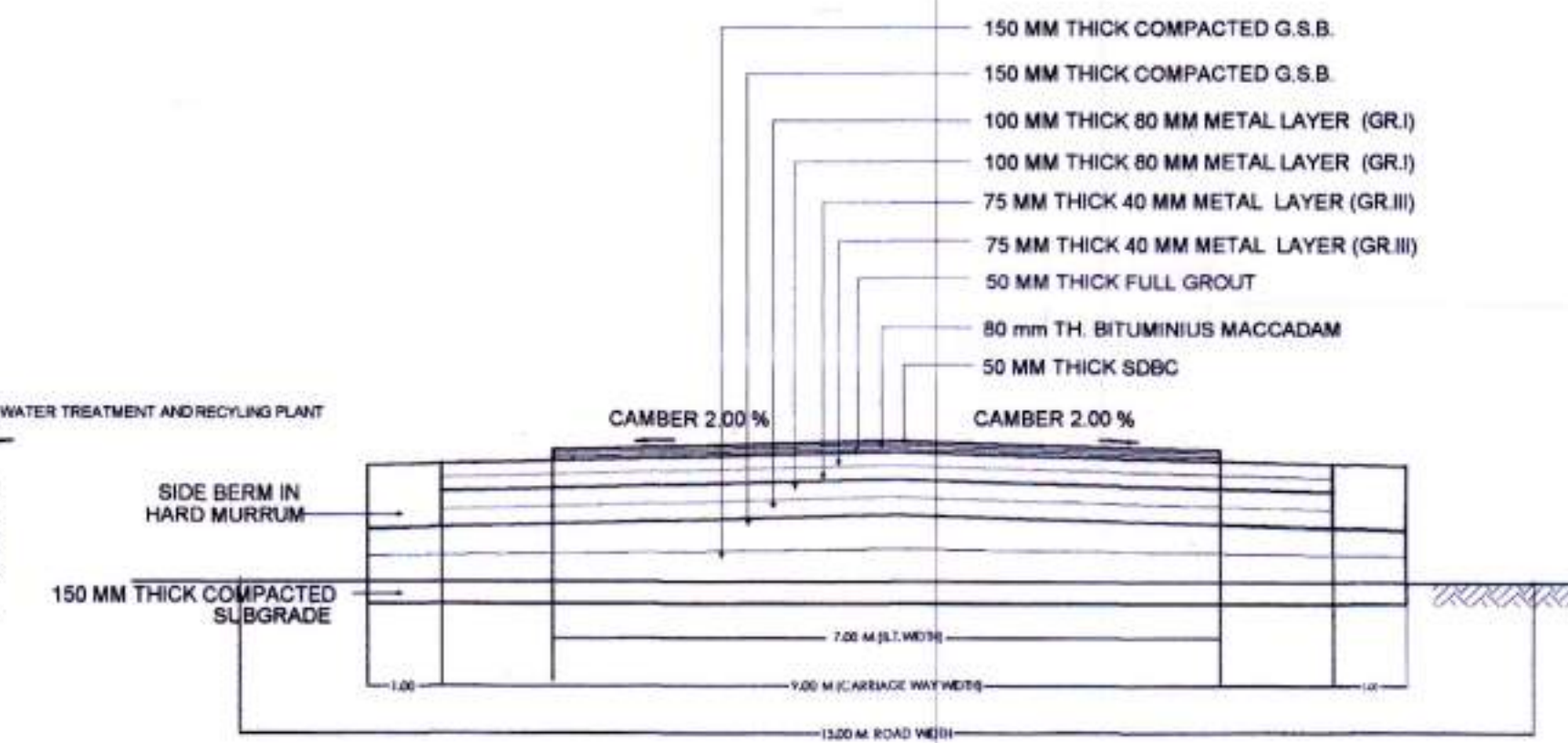
CROSS SECTION OF 15.00 M WIDE ROAD
