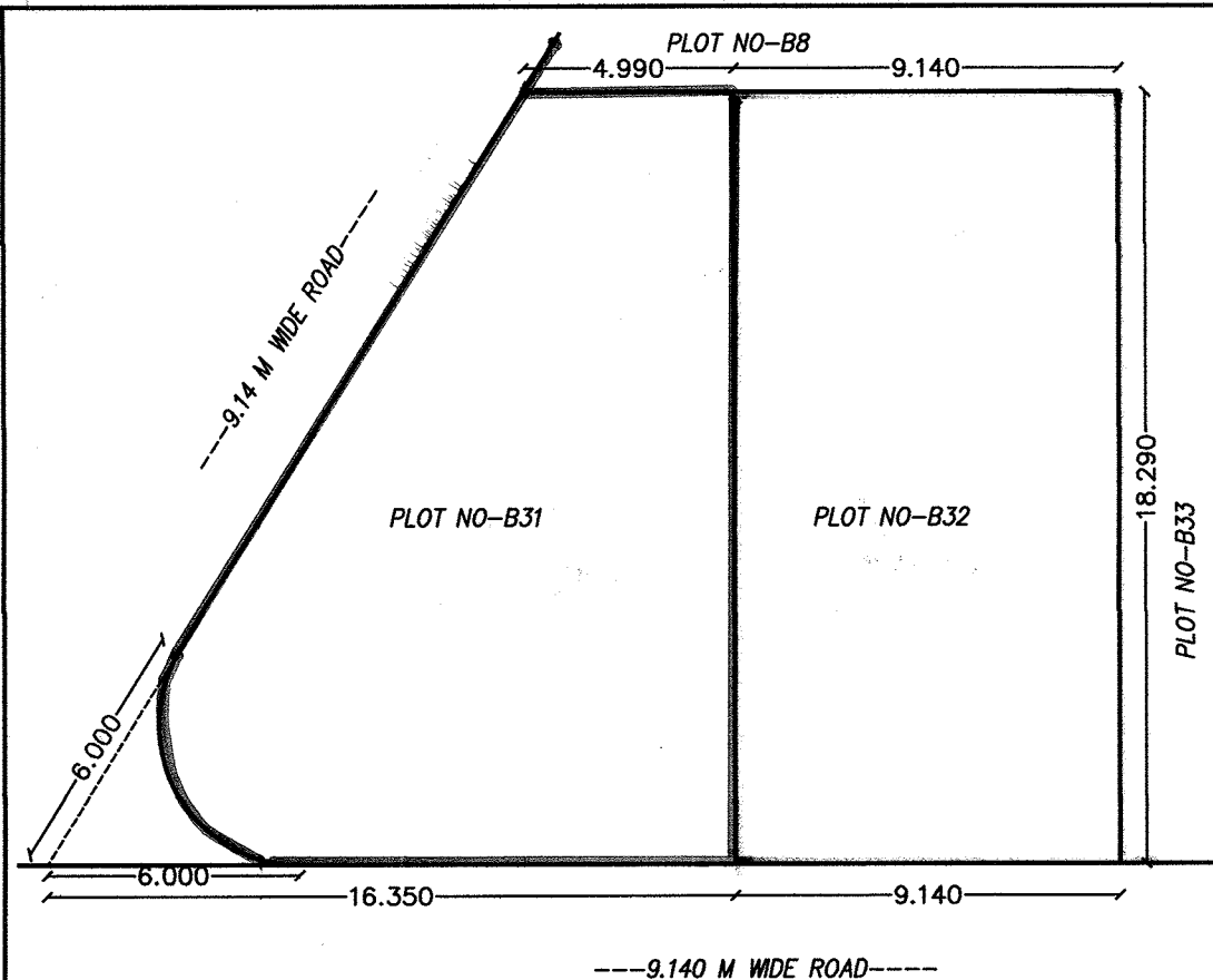
AMALGAMATION PLAN(BEFORE) (SCALE-1:200)
