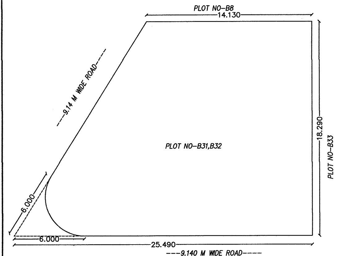
SITE PLAN (AFTTER) (SCALE-1:200)
