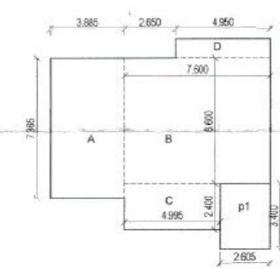
GROUND FL. BLOCK PLAN scale-1:200
