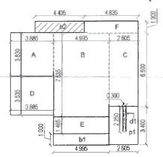
FIRST FL. BLOCK PLAN scale-1:200
