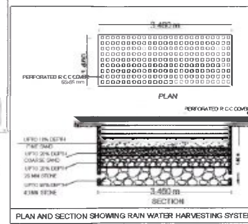
PLAN AND SECTION SHOWING RAIN WATER HARVESTING SYSTEM
