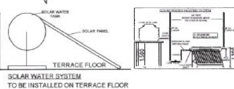
SOLAR WATER SYSTEM TO BE INSTALLED ON TERRACE FLOOR
