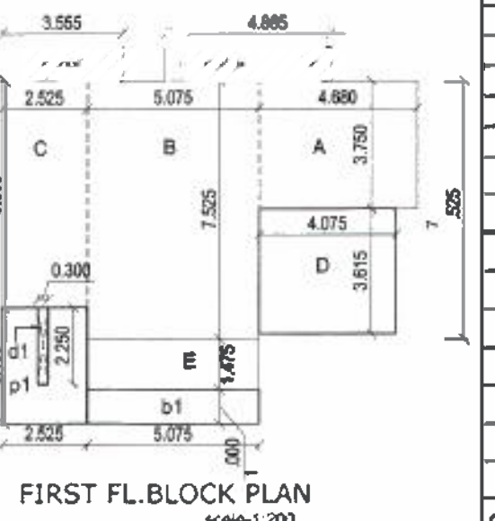
FIRST FL. BLOCK PLAN SCALE - 1:200
