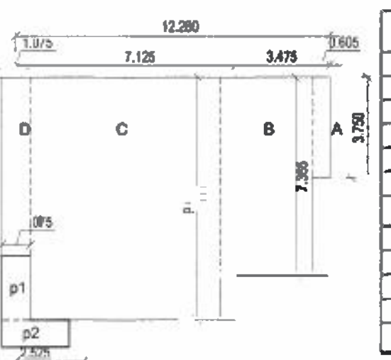
GROUND FL. BLOCK PLAN SCALE - 1:200
