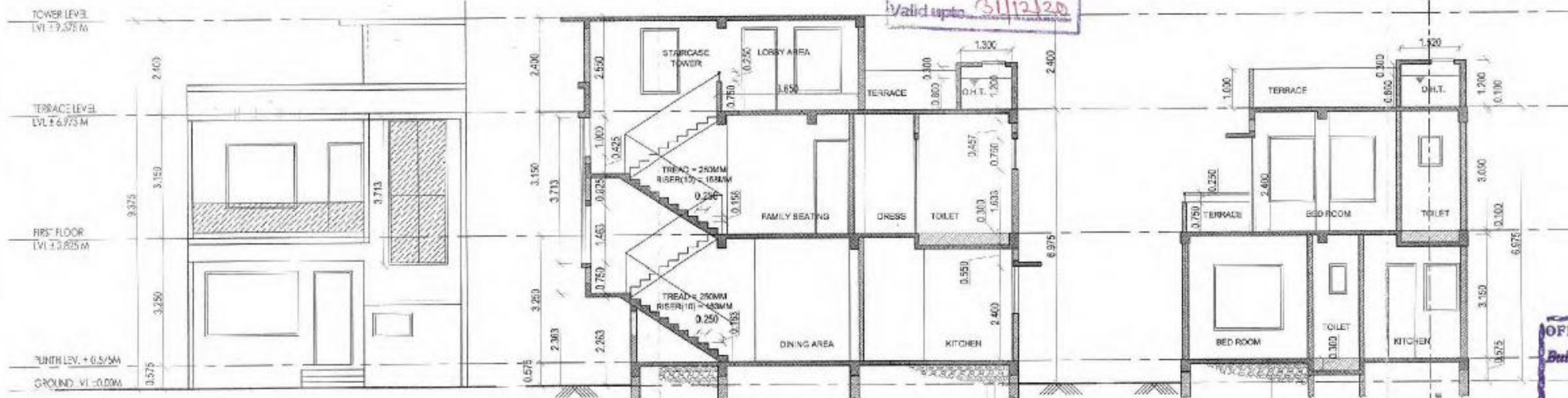
FRONT ELEVATION SCALE - 1:100
