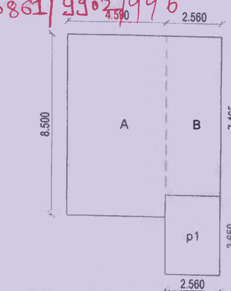
GROUND FL. BLOCK PLAN scale-1:200
