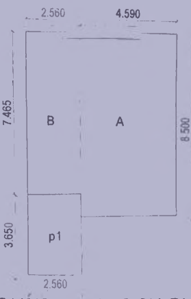
GROUND FL. BLOCK PLAN scale-1:200
