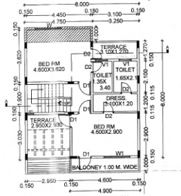
FIRST FLOOR PLAN (SCALE 1:100)
