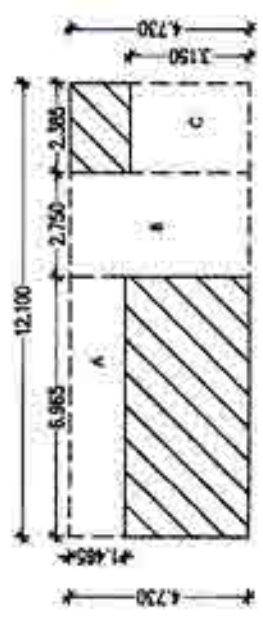
EXISTING GROUND FLOOR BLOCK PLAN (WING - A)
