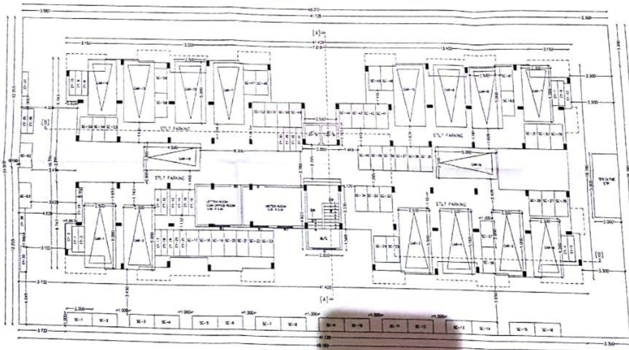
PROP. GROUND FLOOR PLAN (SCALE 1/8")
