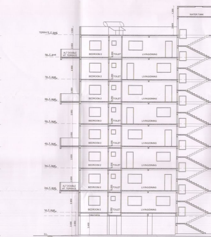
SECTION 1-1 SCALE 1:100
