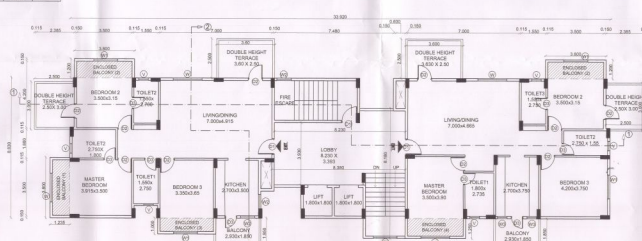
2nd / 4th / 6th / 8th FLOOR PLAN
