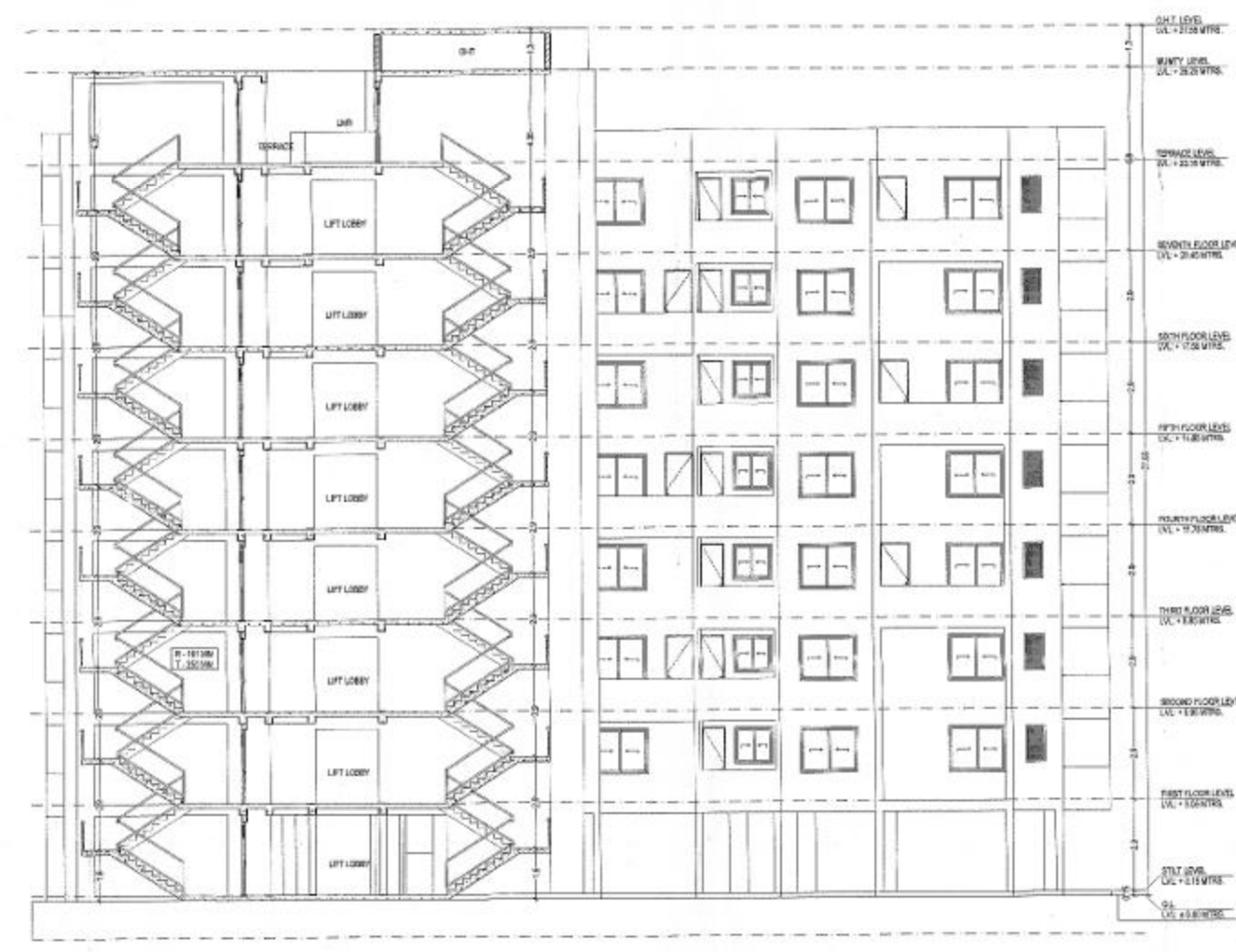
SECTION S - A02
