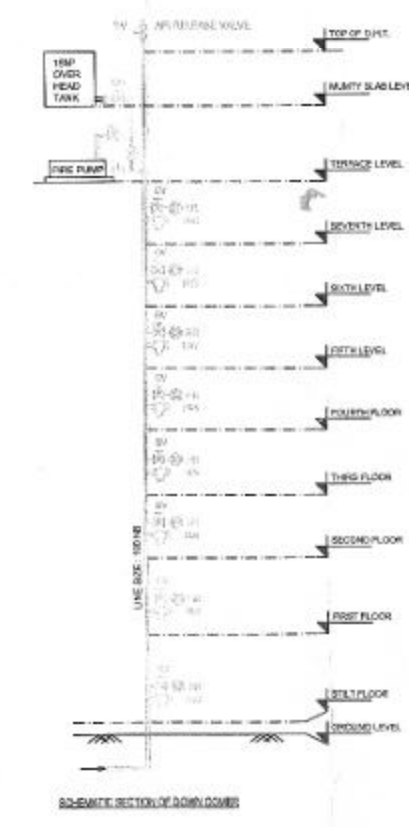
SCHEMATIC SECTION OF DOWN COMES
