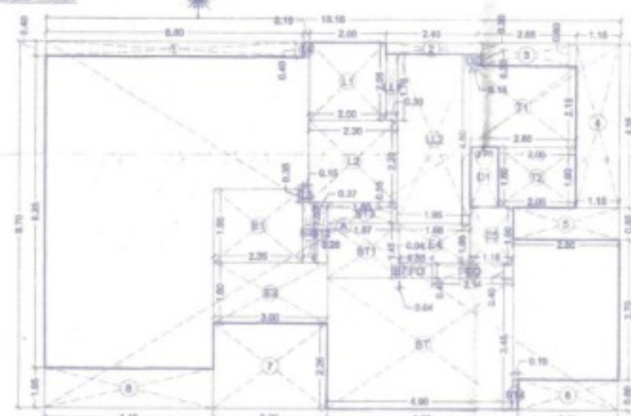
GROUND FLOOR AREA DIAGRAM SCALE - 1:100
