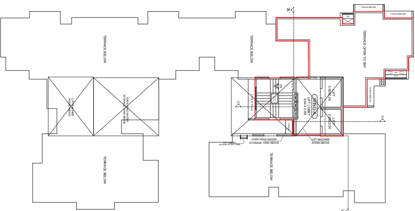
TERRACE FLOOR PLAN (WING-A & WING-B)
