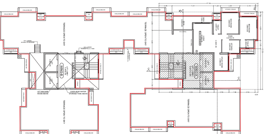
15TH (PT) FLOOR PLAN (WING-A & WING-B) SCALE - 1/100
