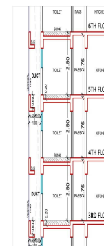
SECTION THROUGH TOILET SERVICE DUCT
