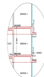
SECTION THROUGH WINDOW CORNICE
