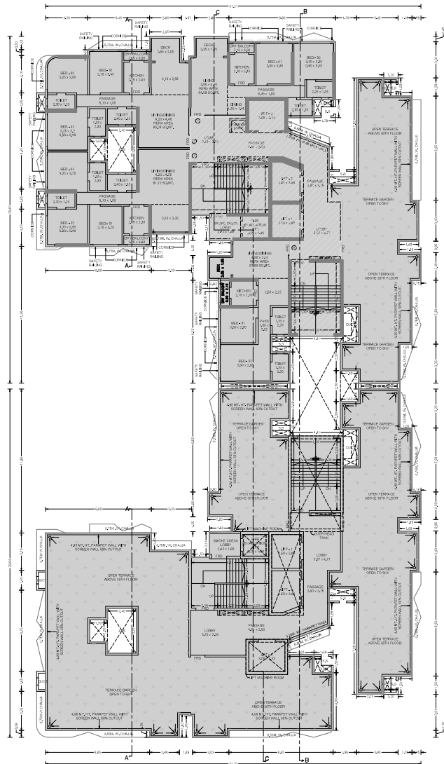
31ST FLOOR PLAN
