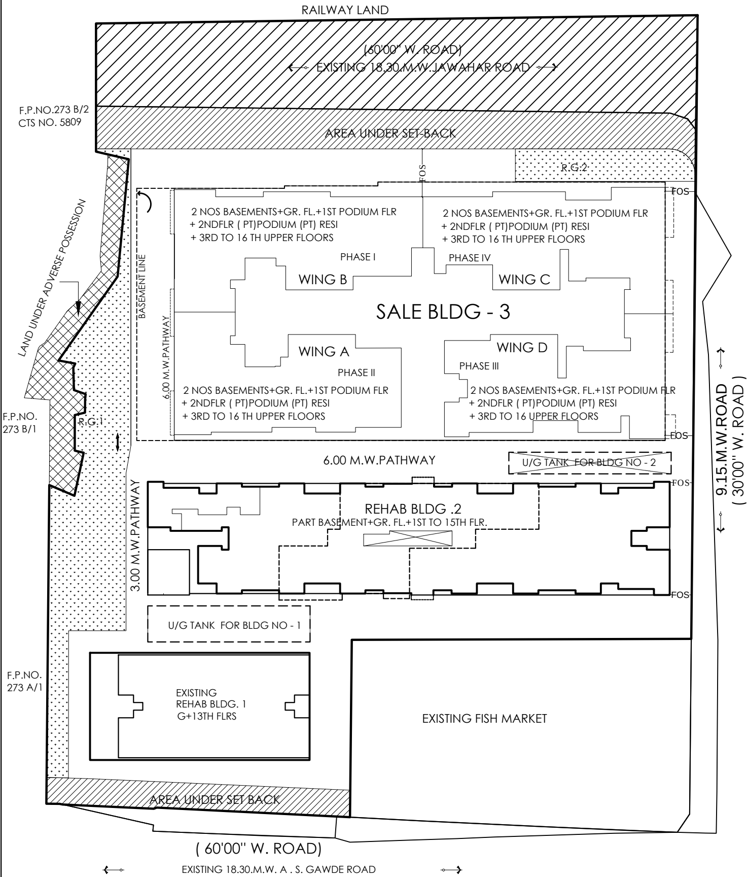
PROPOSED LAYOUT PLAN
