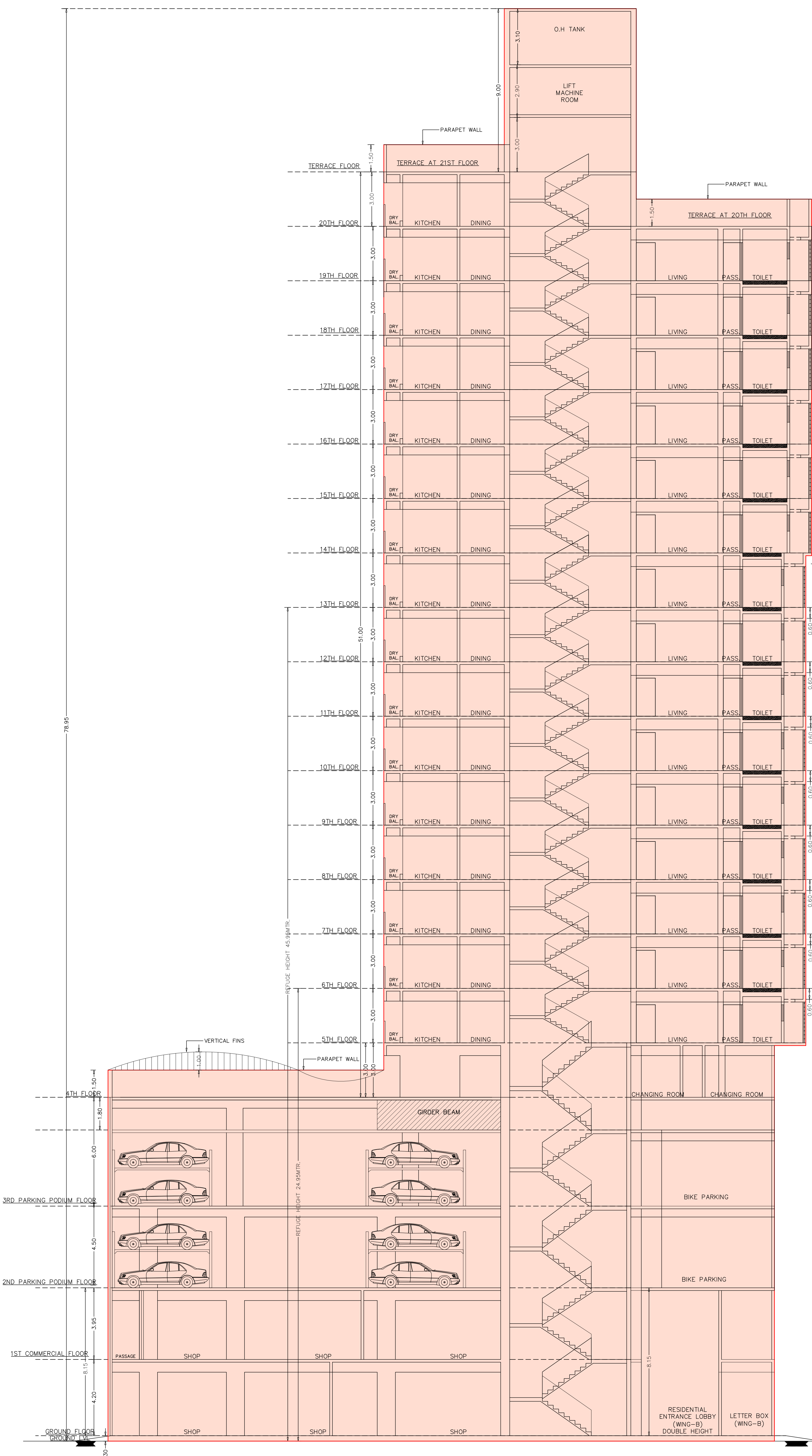
SECTION B-B SCALE = 1:100
