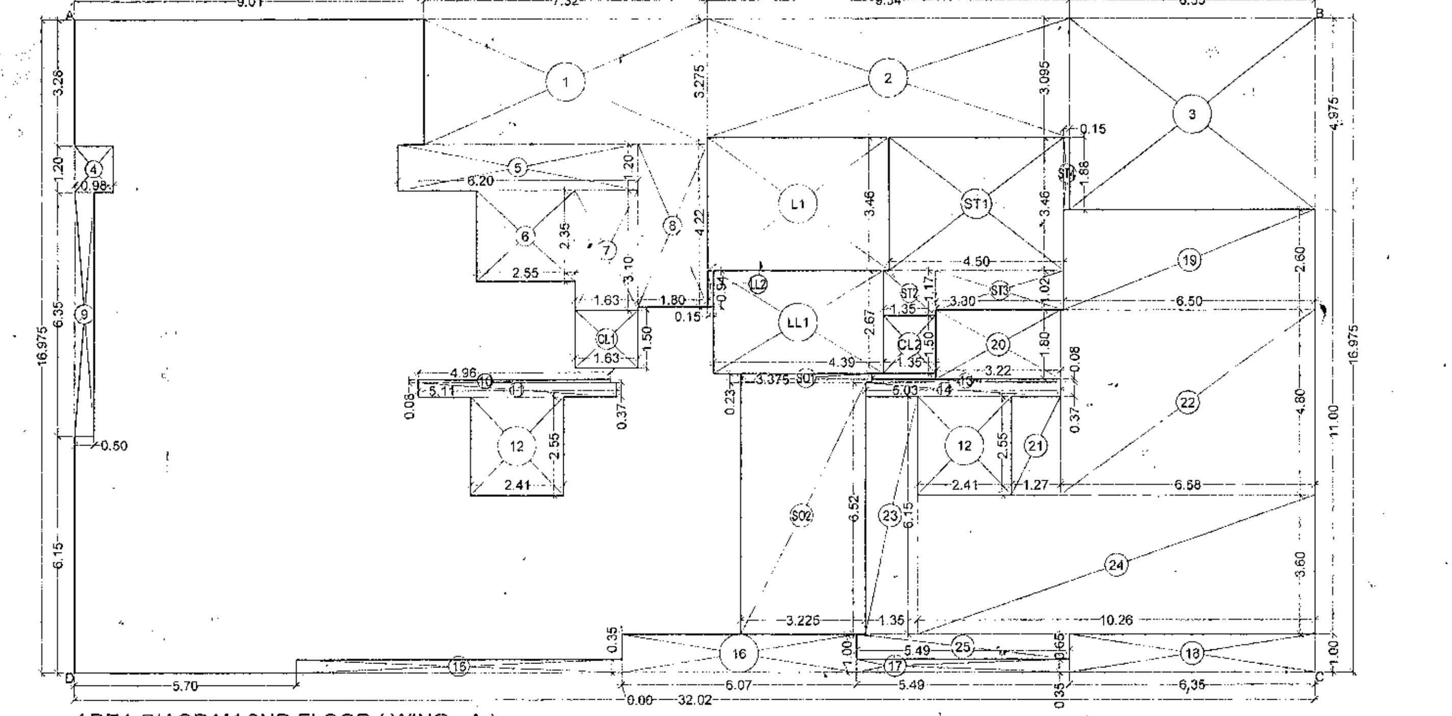
AREA DIAGRAM 2ND FLOOR (WING - A)
