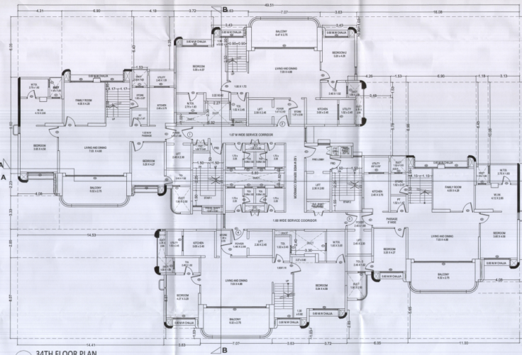
T34 34TH FLOOR PLAN (SCALE - 1:300)
