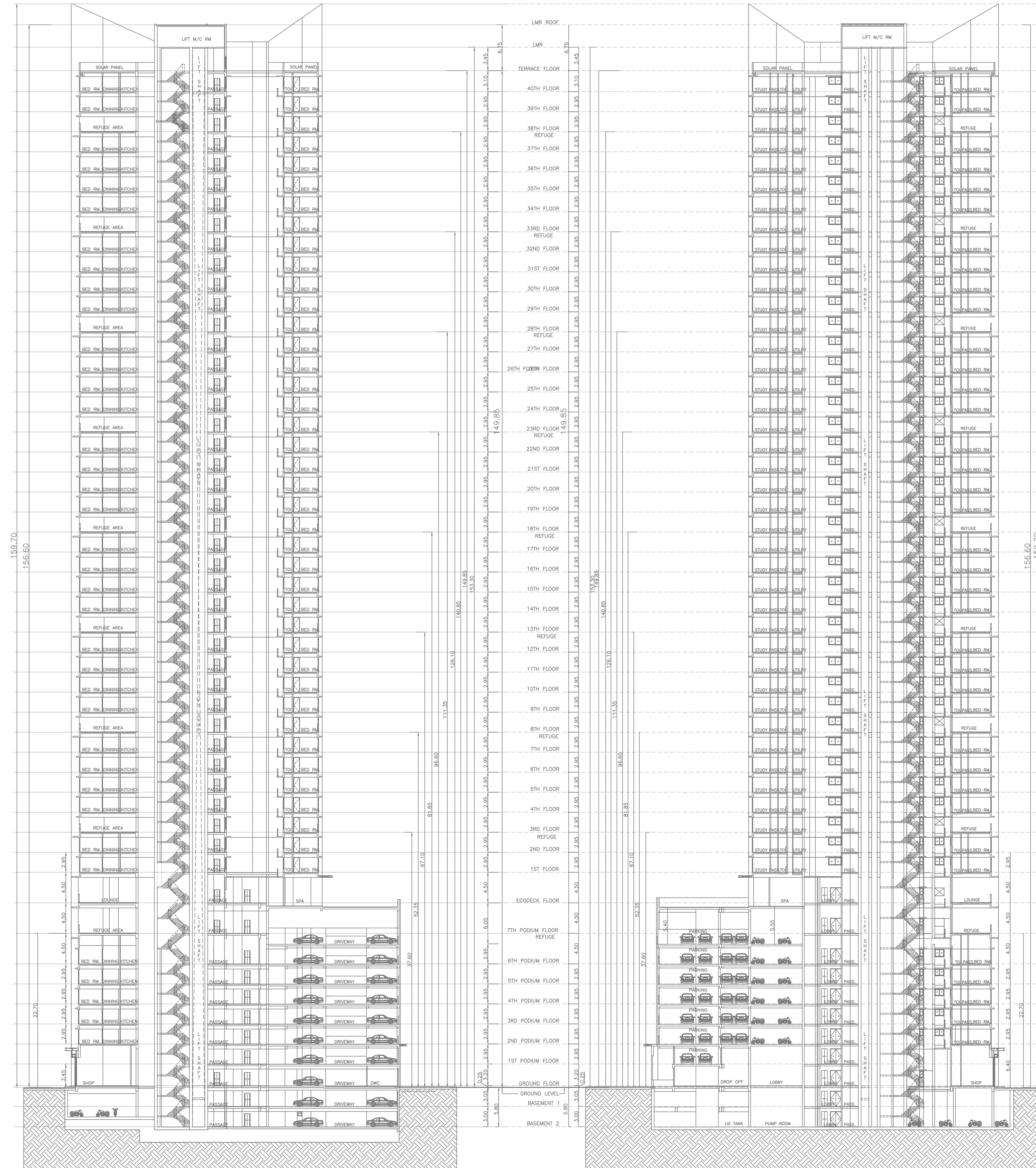
SECTION A - A TOWER - B SCALE = 1:250
