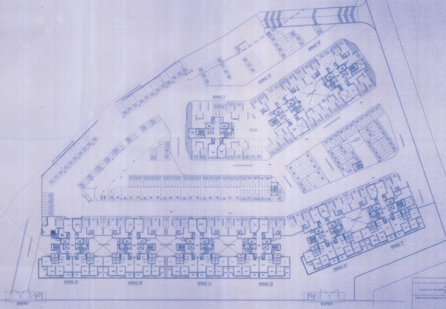
FIRST FLOOR PODIUM PLAN SCALE-1:250
