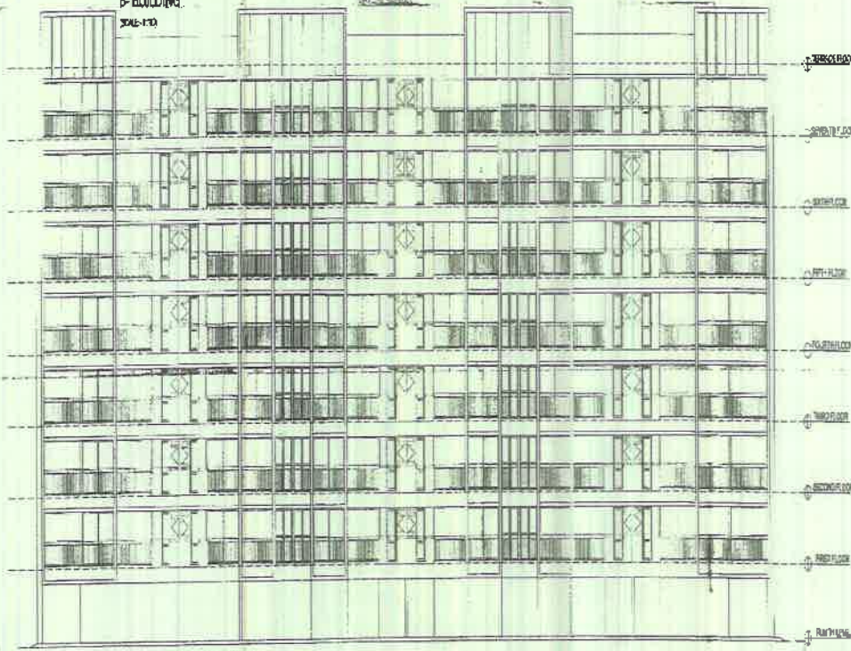
FRONT ELEVATION OF B-BUILDING SCALE-1:10
