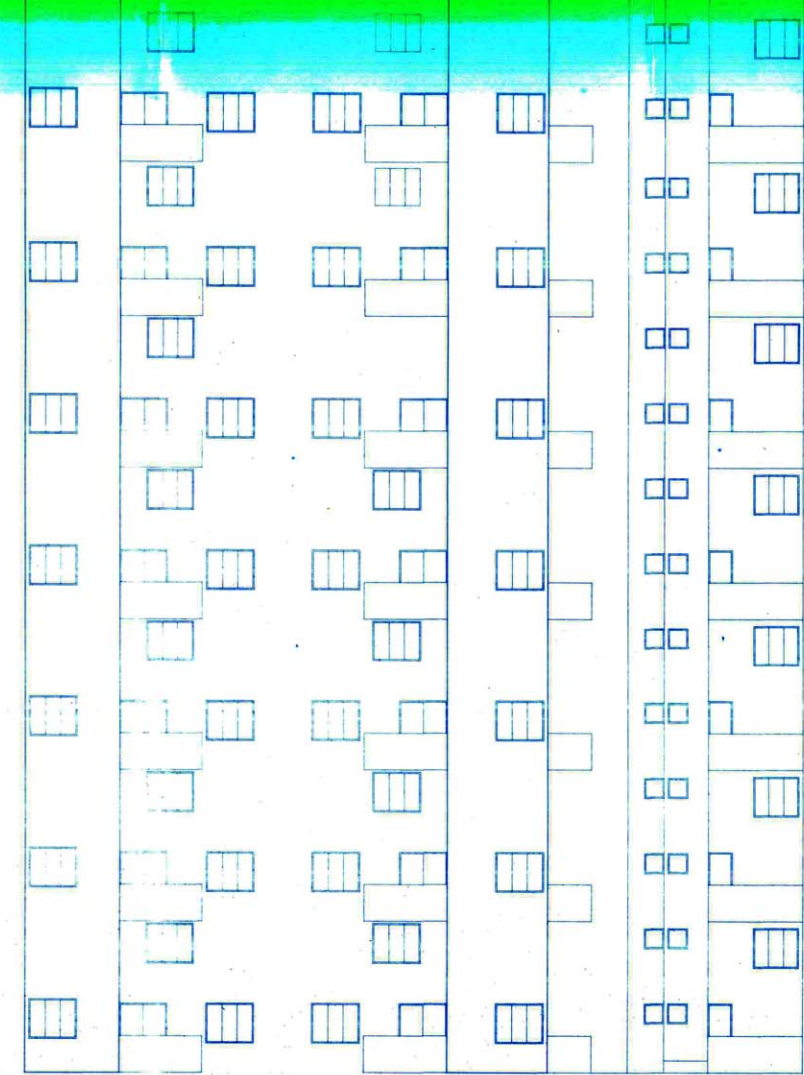
BUILDING -B ELEVATION SCALE 1:100
