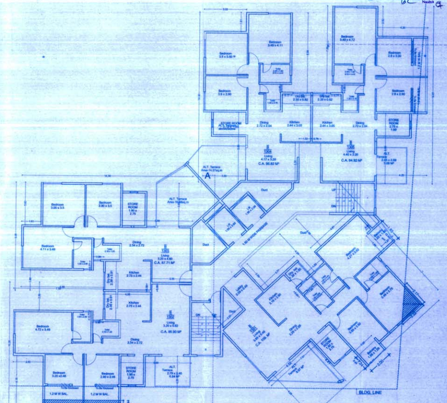
BUILDING-B 13 FLOOR PLAN
