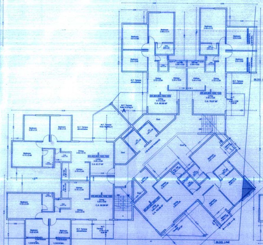
BUILDING-B 2,4,6,10,12 FLOOR PLAN
