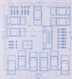
PARKING PLANS
