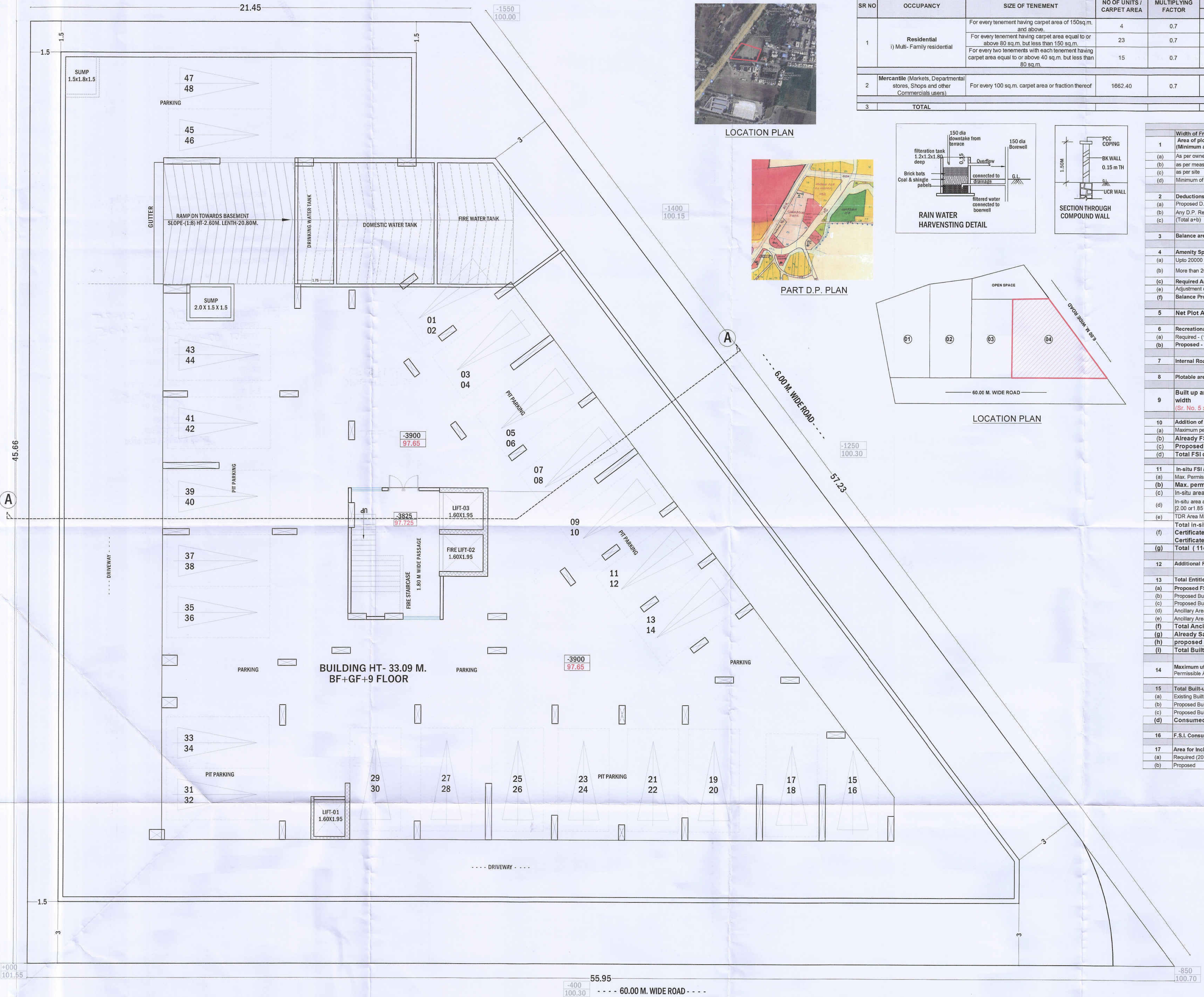
BASEMENT FLOOR PLAN
