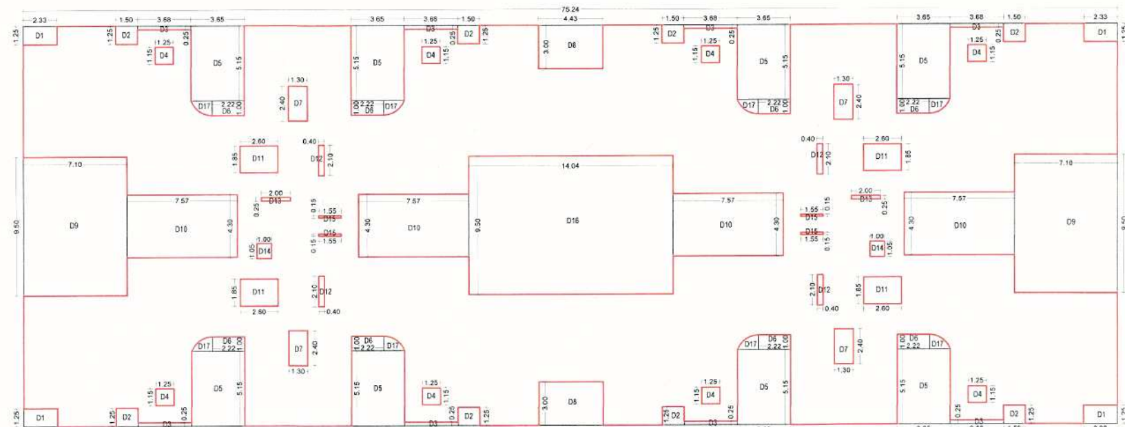
TWENTY FIRST FLOOR P-LINE BLOCK PLAN
