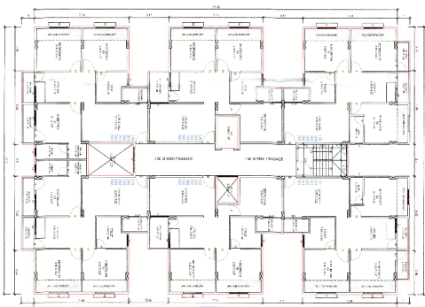
TYPICAL PLAN OF FIRST TO SIXTH FLOOR
