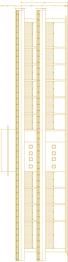
WEST SIDE ELEVATION
