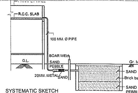
SECTIONAL DETAILS OF RAIN WATER HARVESTING
