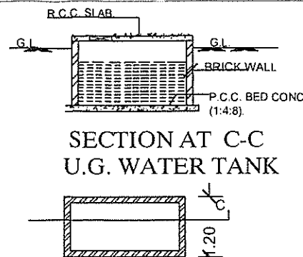
PLAN OF U.G. WATER TANK.
