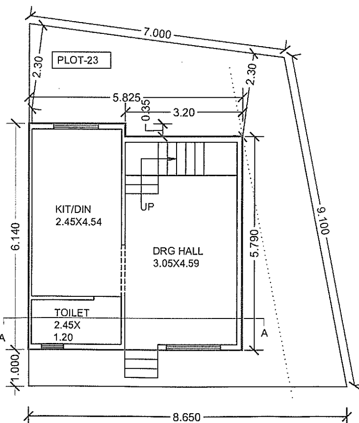
GROUND FLOOR PLAN(23)
