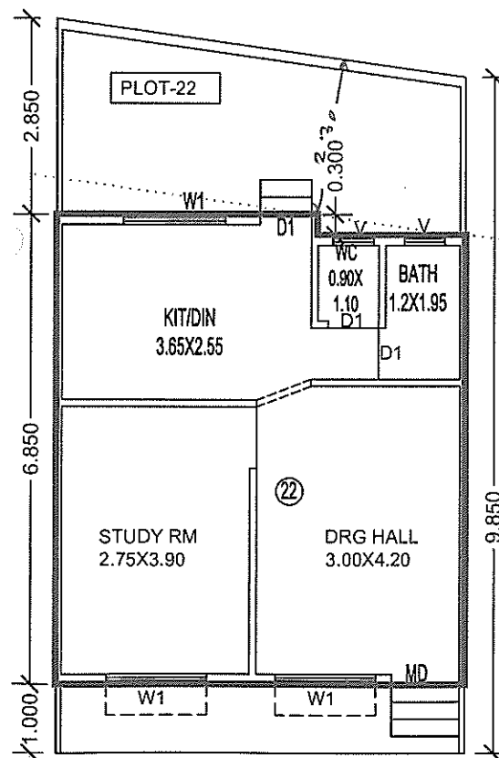
GROUND FLOOR PLAN(22)
