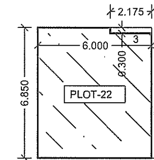
GR.FL BLOCK PLAN(P-22) OVER ALL DIM 6.00X6.85=41.10 SQM LESS 1)2.175X0.30 =0.652 SQM NET =40.448 SQM
