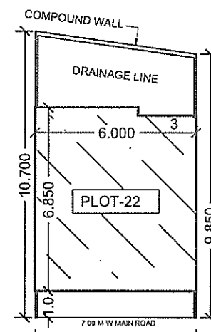
BLOCK PLAN(22)
