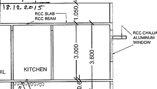
TYPICAL SECTION (21)
