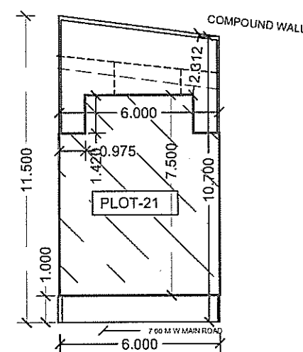
BLOCK PLAN (21)
