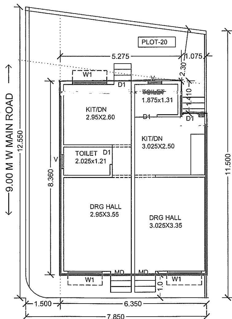
GROUND FLOOR PLAN (20)
