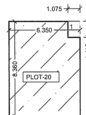
GR.FL BLOCK PLAN(P-20) OVER ALL DIM 6.35X8.36 =53.086 SQM LESS 1) 1.075X1.41 = 1.515 SQM NET GR FL. =51.571 SQM
