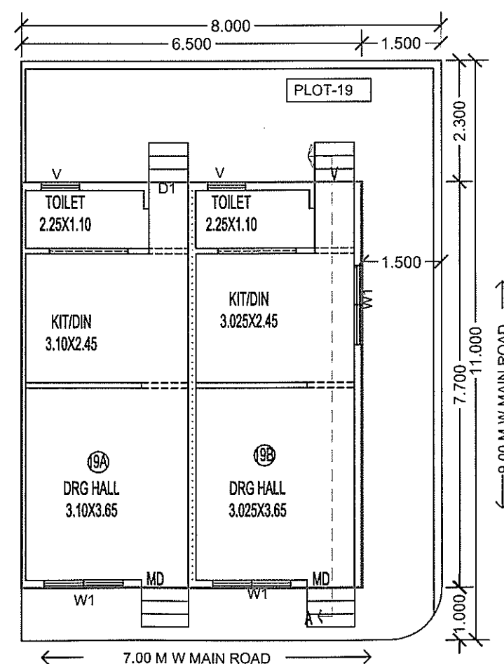
GROUND FLOOR PLAN (19)
