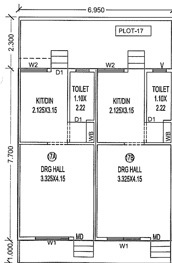
GROUND FLOOR PLAN(17) SCALE 1:100
