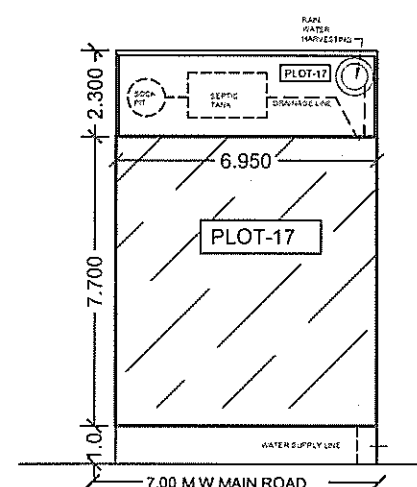
BLOCK PLAN(17)
