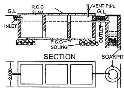
PLAN TYPICAL SEPTIC TANK & SOAK PIT DETAILS
