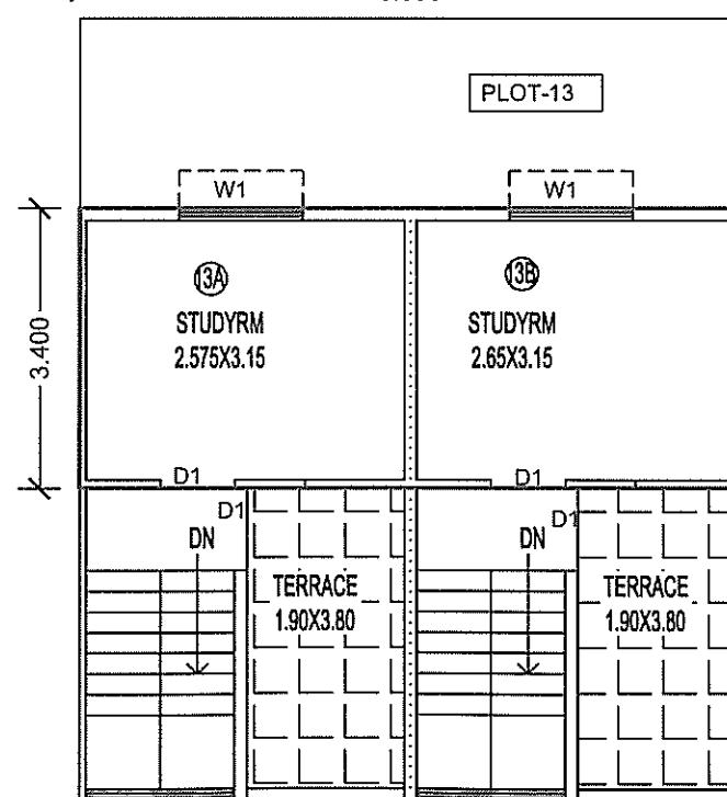
FIRST FLOOR PLAN (13)
