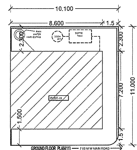
GROUND FLOOR PLAN(11) ← 7.00 M W MAIN ROAD
