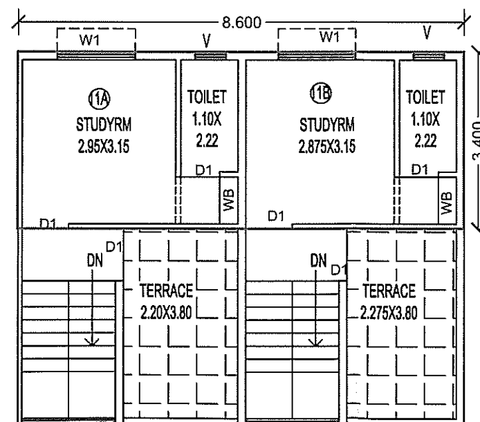
FIRST FLOOR PLAN(11)
