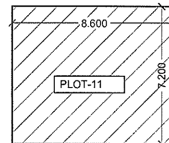
GR.FL BLOCK PLAN(P-11) OVER ALL DIM 8.60X7.20 =61.92 SQM
