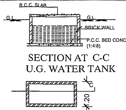
PLAN OF U.G. WATER TANK.
