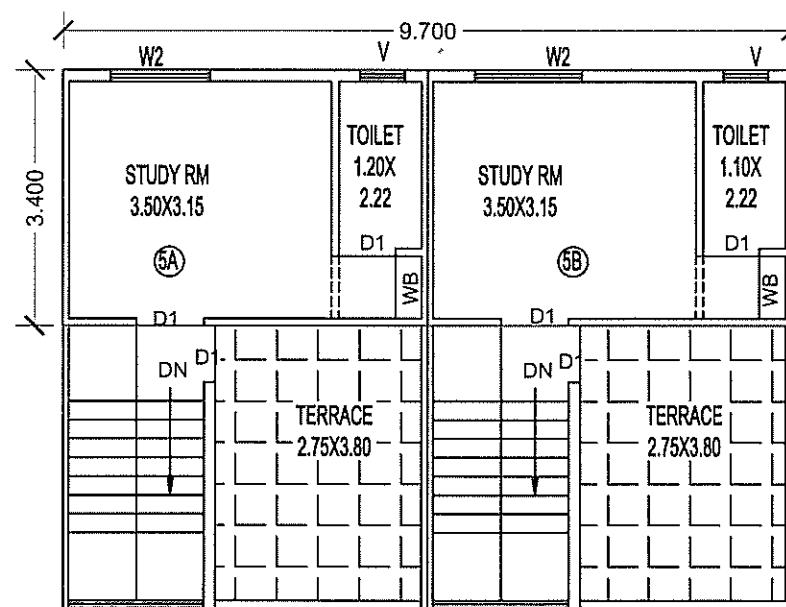
FIRST FLOOR PLAN (5)
