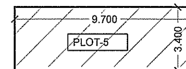
FIRST.FL BLOCK PLAN(P-5) OVER ALL DIM 9.70X3.40 =32.98 SQM
