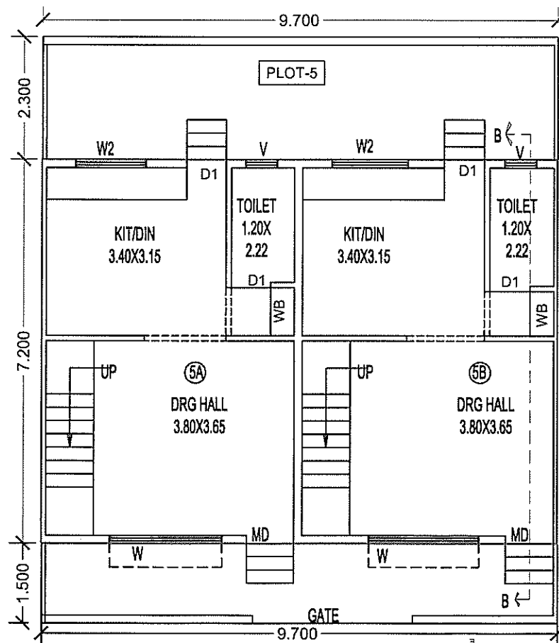
GROUND FLOOR PLAN (5)
