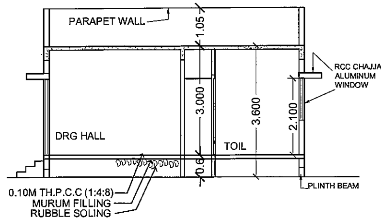
TYPICAL SECTION (3)
