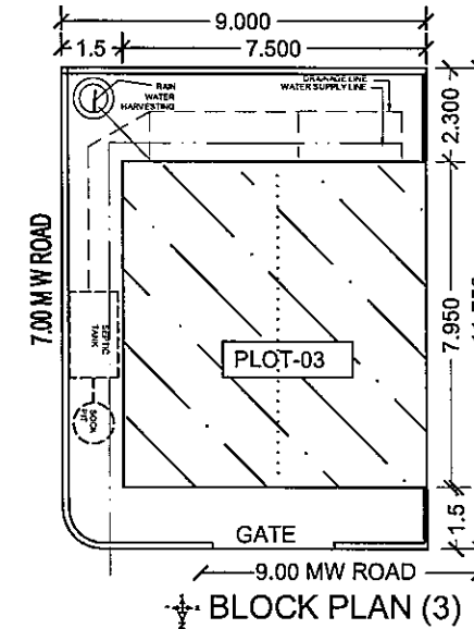
GR.FL BLOCK PLAN(P-03) OVER ALL DIM 7.50X7.95=59.625 SQM
